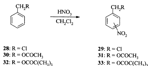
Scheme 10
