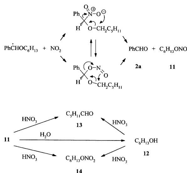
Scheme 6
